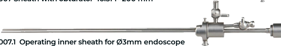
BG2007 Sheath with obturator 16.5Frx200 mm
